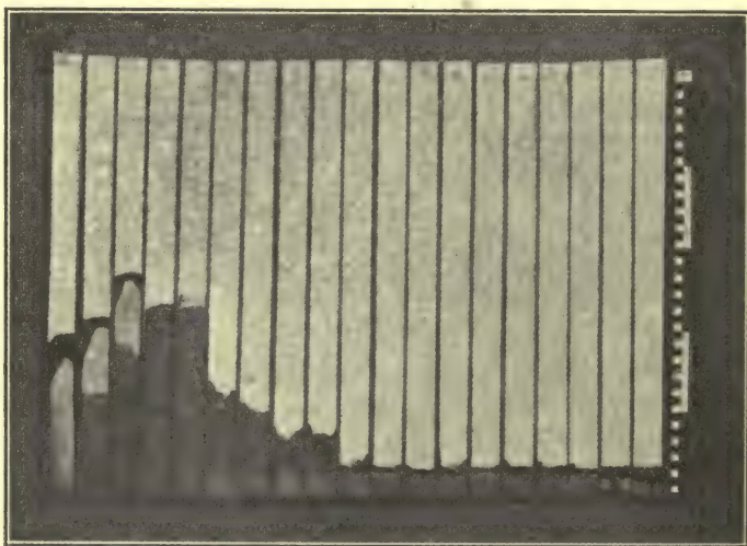
FIG. 51.—Dialysis of a ferric nitrate solution. (According to N. Sahlbom. )
